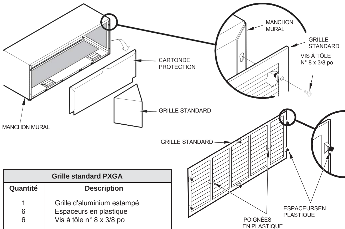
Figure 13 Grille standard
