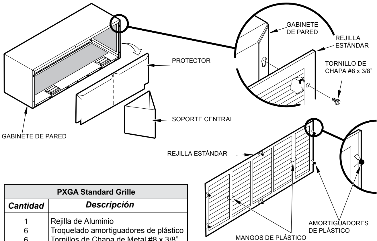
Figure 13 Standard Grille
