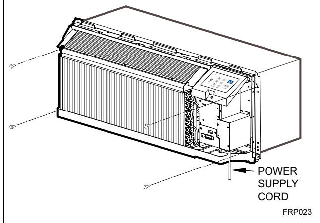
Figure 23 Securing Unit
